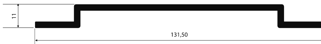
NI-791 1,196 kg/m
