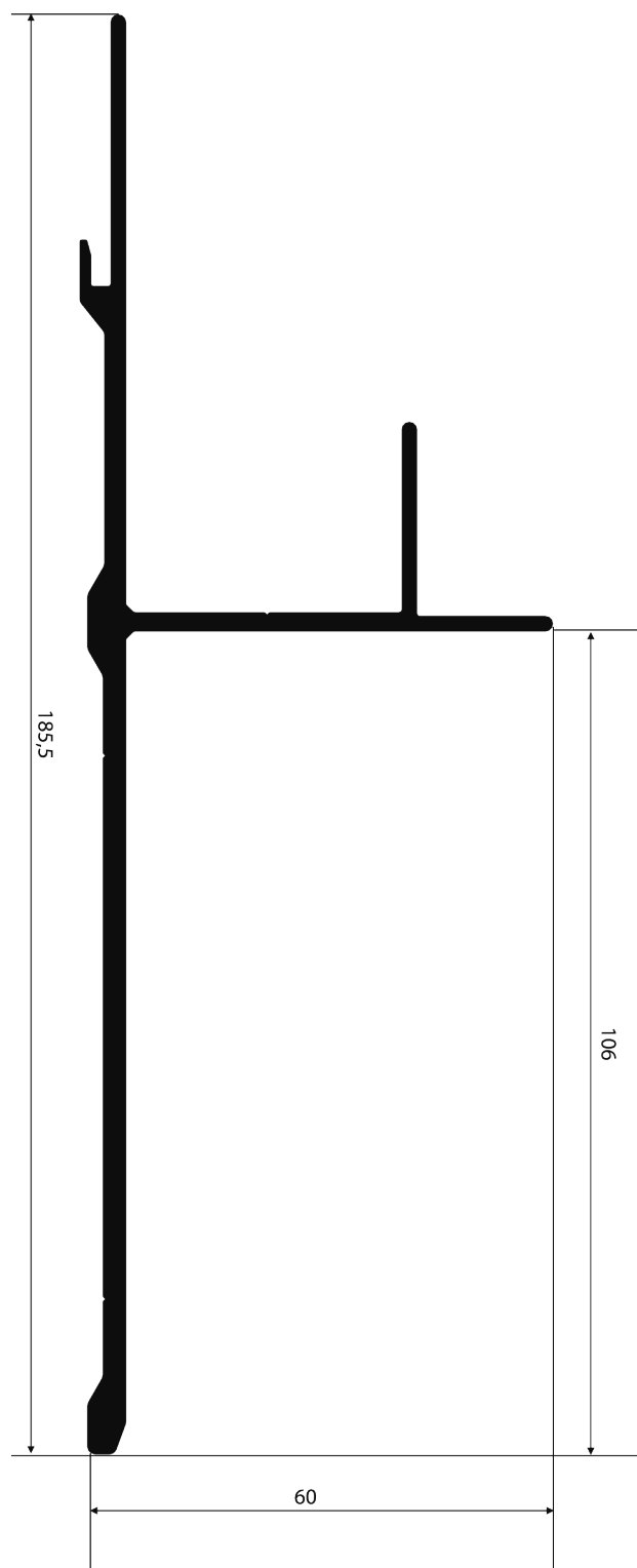
NI-414 2,025 kg/m
