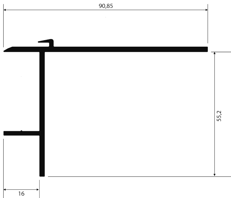
NI-364 1,046 kg/m
