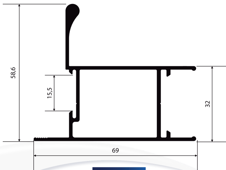
LG-017 1,004 Kg/m
