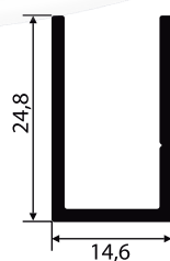
U-555M 0,260 Kg/m
