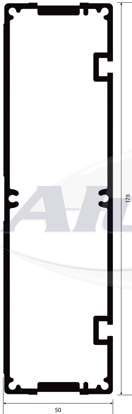
NI-122 3,573 Kg/m
