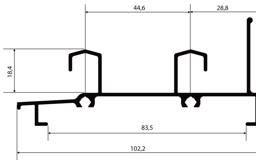
LG-047 1,133 Kg/m
