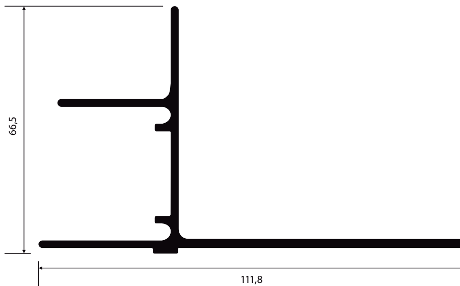
NI-210 1,295 Kg/m
