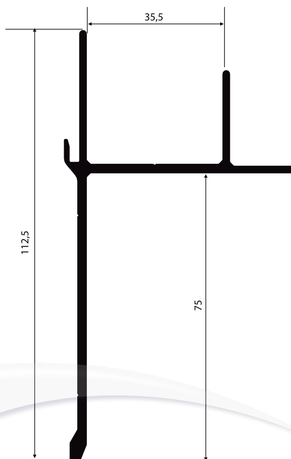
NI-420 1,264 Kg/m
