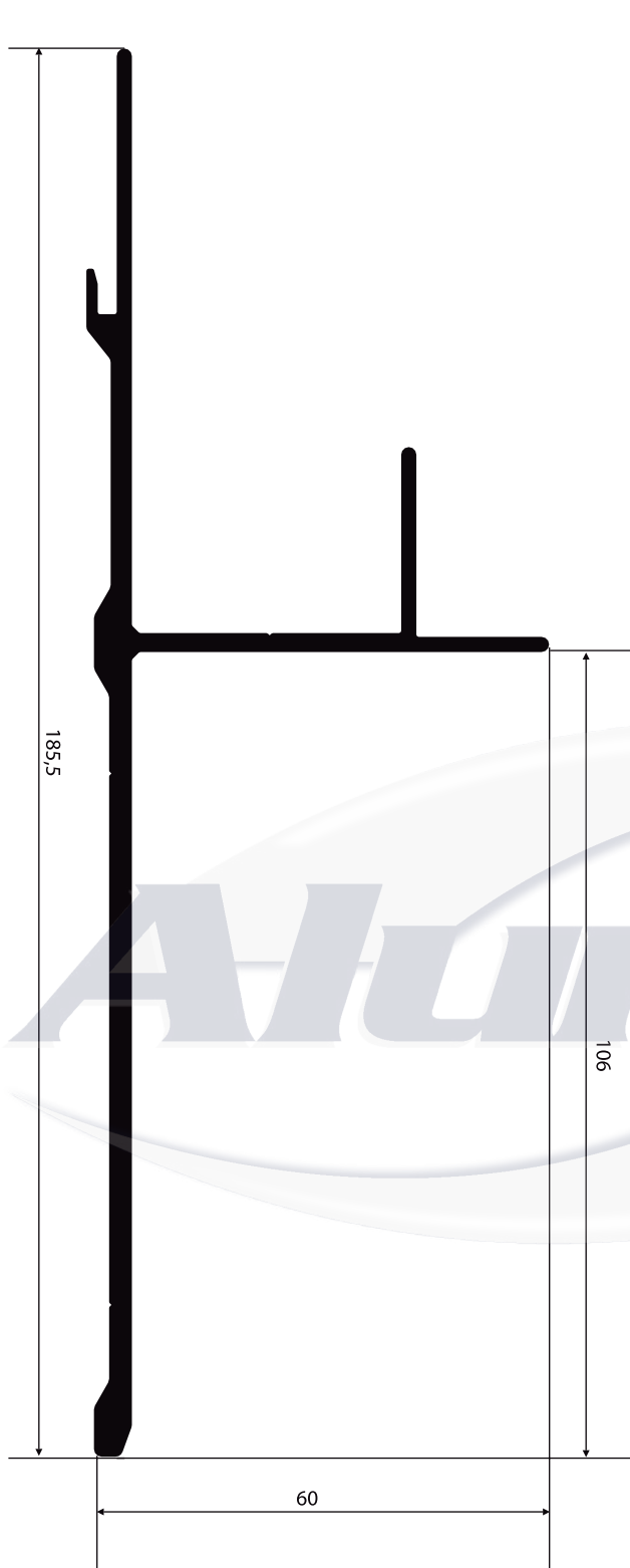
NI-414 2,025 Kg/m
