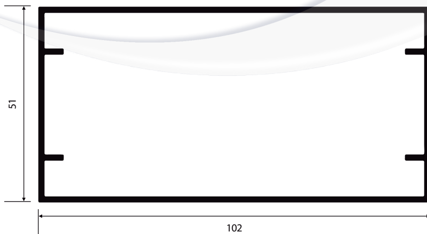
TUB-4598 1,385 Kg/m
