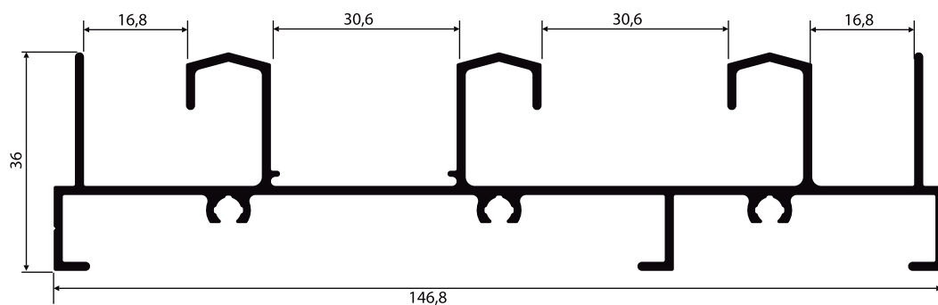
NI-519 1,620 Kg/m
