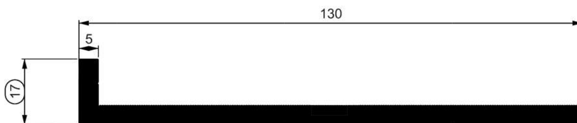
NI-2454 1,902 Kg/m
