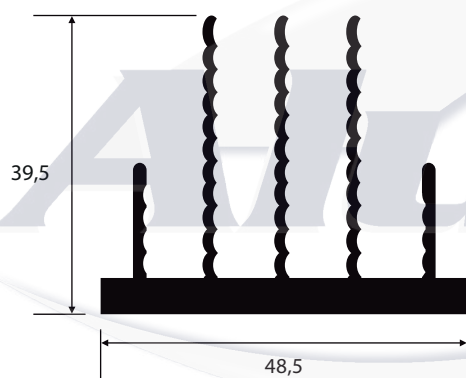
NI-068 1,158 Kg/m
