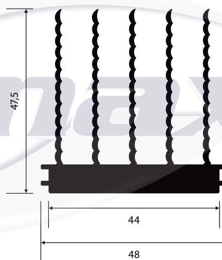
NI-123 1,726 Kg/m
